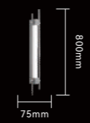
6311/YELLOW+CH 800mm Item Size: L800*W75mm Power: LED 15W
